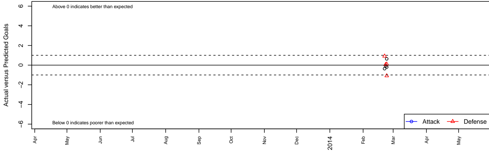
Sereno West 00 White B99 Dots are actual minus expected GF (blue circles) and GA (red triangles). Blue line is smoothed change in attack strength. Red is smoothed change in defense strength.
